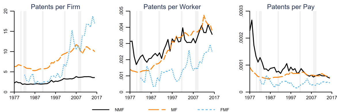
Figure 5: Patent Efficiency
