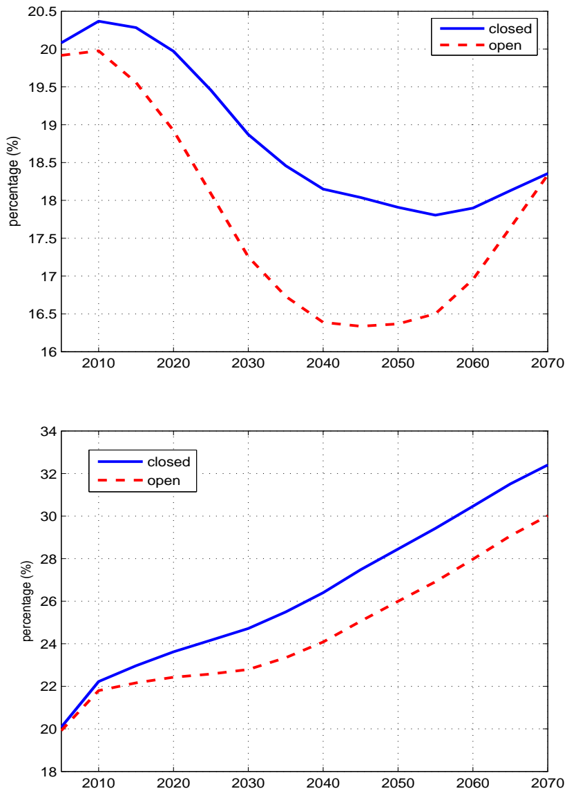
Figure 4: The path of equilibrium saving rates in closed and open economy
