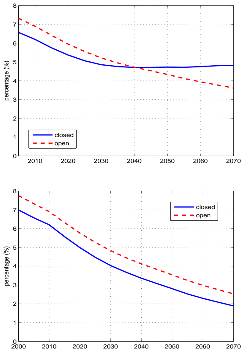
Figure 5: The path of equilibrium interest rates in closed and open economy
