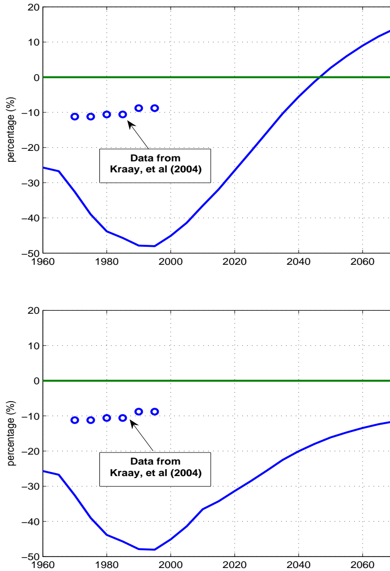
Figure 6: The path of equilibrium external wealth in open economy
